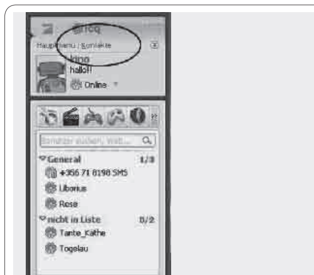
ICQ Messenger
